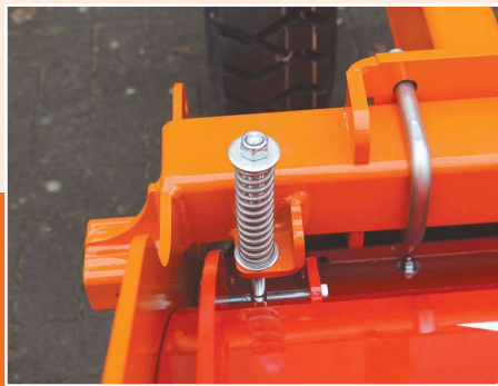
Self-cleaning hood
